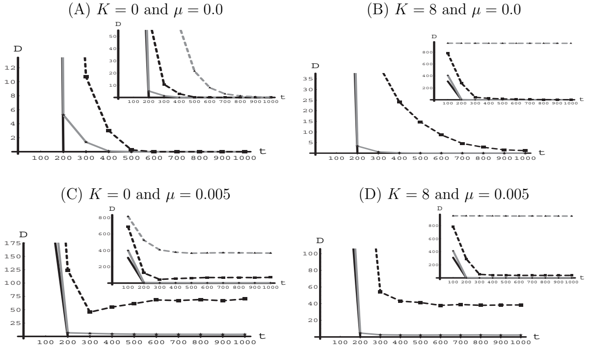
Figure 4: The diversity within an organization for two levels of complexity, K = 0 (left) and K = 8 (right), and two degrees of environmental uncertainty, \mu = 0.0 (top) and \mu = 0.005 (bottom). The communication is active ( p = 1.0 ). Four values of \lambda are considered: \lambda = 0.0 (solid black), \lambda = 0.2 (solid gray), \lambda = 0.6 (dashed black), \lambda = 1.0 (dashed gray). For the clarity of exposition, only \lambda \in \{0.0, 0.2, 0.6\} are shown in the main figure. See the insets for all the four \lambda s. The extent of diversity is measured based on the discrepancy between individual configurations and their means. The data is generated by taking the average per period diversity for each block of 100 periods. The average from 100 simulation runs is reported.
